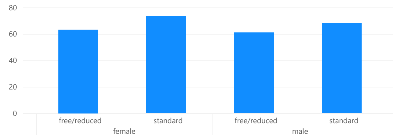
Average Score
